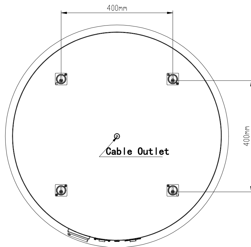
REAR VIEW
