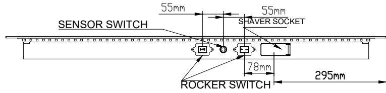
BOTTOM VIEW
