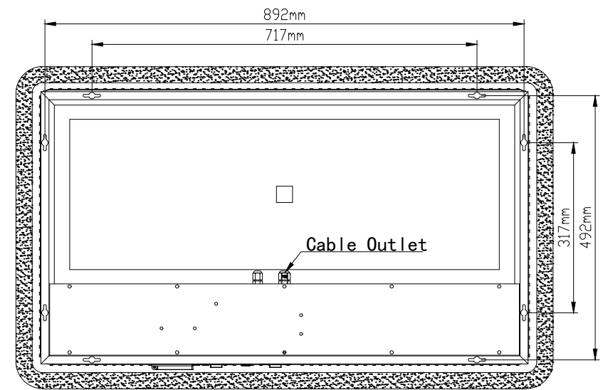
REAR VIEW
